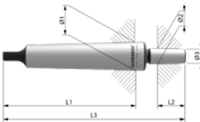
Arbors DIN-238 taper
