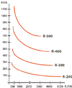
AXIAL LOAD 2.000 hours tool life
