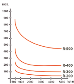
RADIAL LOAD 2.000 hours tool life
