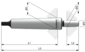
Arbors Jacobs taper
